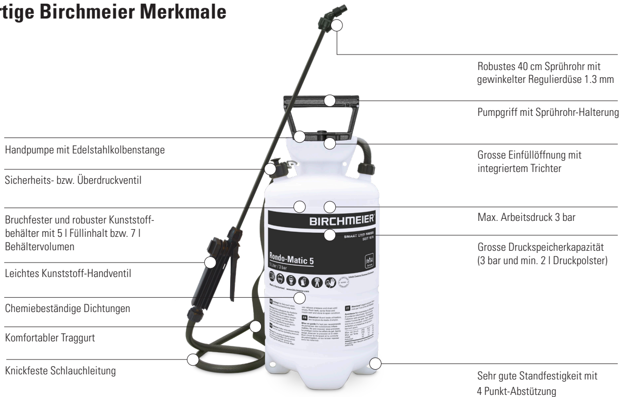
Rondo-Matic 5 Art.Nr. 11622101
